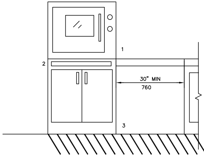
(a) SIDE-HINGED DOOR
